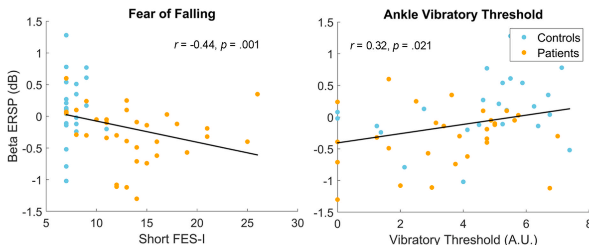
Fig. 3. Correlations between high-beta (19–24 Hz) between –250 to –150 ms prior to peak instability and concerns about falling (short Falls Efficacy Scale—International [FES-I]; left) and ankle vibratory perceptual thresholds (arbitrary units; right). Note, higher scores for the short FES-I indicate greater concerns (or, ‘fears’) about falling, whilst higher vibratory threshold scores indicate greater (i.e., better) ankle vibratory perception.
