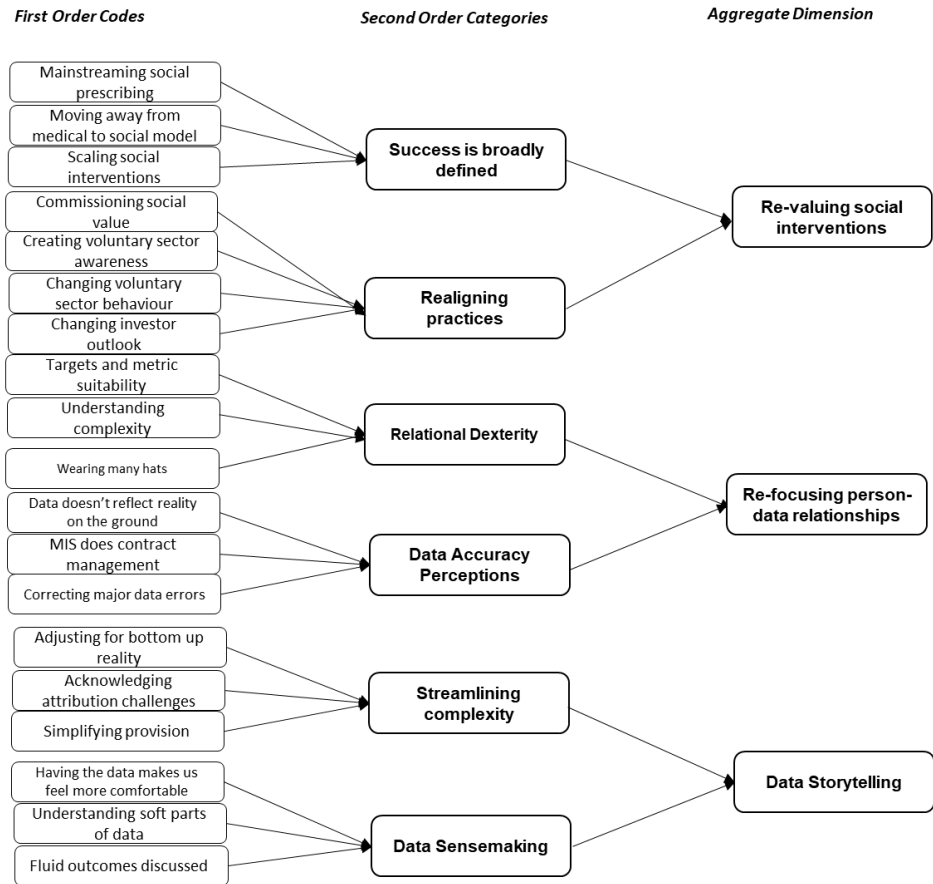
Figure 1. Data Structure
