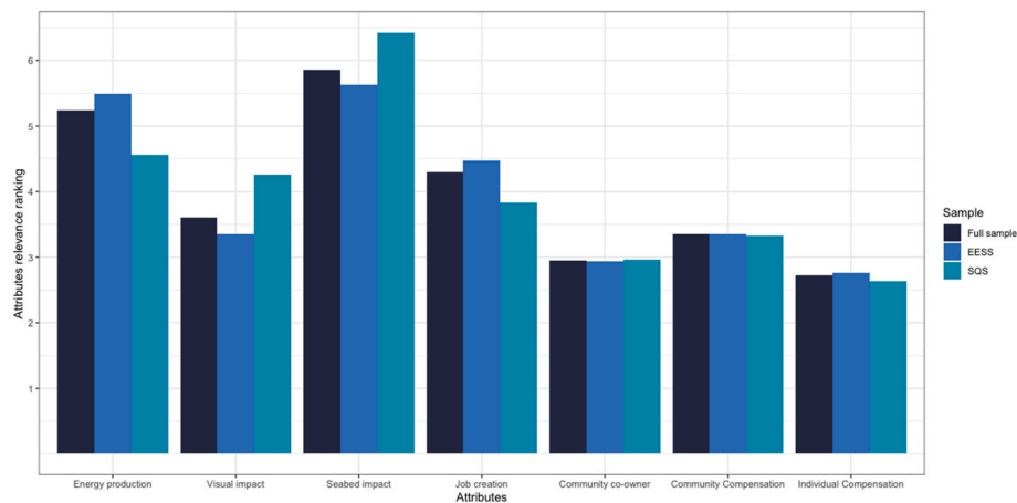
Fig. 2. Attributes ranking.
