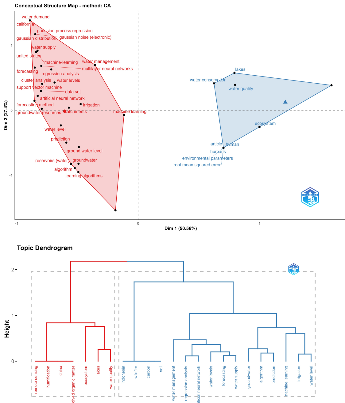
Figure 12. Conceptual structure and dendrogram for a forecasting water levels topic.
