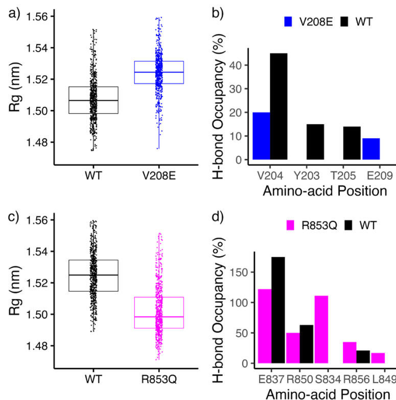
Figure 6 a) Box plot showing the radius of gyration (Rg) of voltage sensing domain 1 for WT (black) and V208E (blue). b) Hydrogen bond occupancy (%) formed between V208 and amino-acids within 3.5 Å distance cutoff of V208: black (WT), blue ( V208E ) c) Radius of gyration of voltage sensing domain 2 for WT (black) and R853Q structure (magenta) d) Hydrogen bond occupancy (%) formed between R853 and amino-acids within 3.5 Å distance cutoff of R853: black (WT), magenta ( R853Q ).
