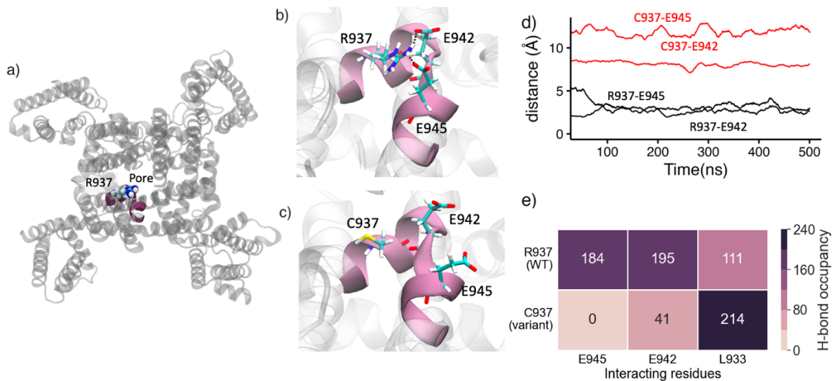
Figure 4 (a) Top view of the NaV1.2 model highlighting the position of R937 in the WT structure. (b) Close-up view showcasing the electrostatic interactions formed between R937 and E942 and E945 in WT. (c) in variant R937C . (d) Simulation time-dependent distance profiles of R937C -E942 and R937C -E945, represented by black (WT) and red lines (C937) respectively, illustrating the differences between the WT and R937C . (e) Heatmap of hydrogen bond occupancy analysis reveals the formation of hydrogen bonds by R937 and C937 with residues within a 3.5 Å cutoff distance.
