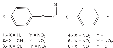
SCHEME 1 Structure of a series of diaryl dithiocarbonates
