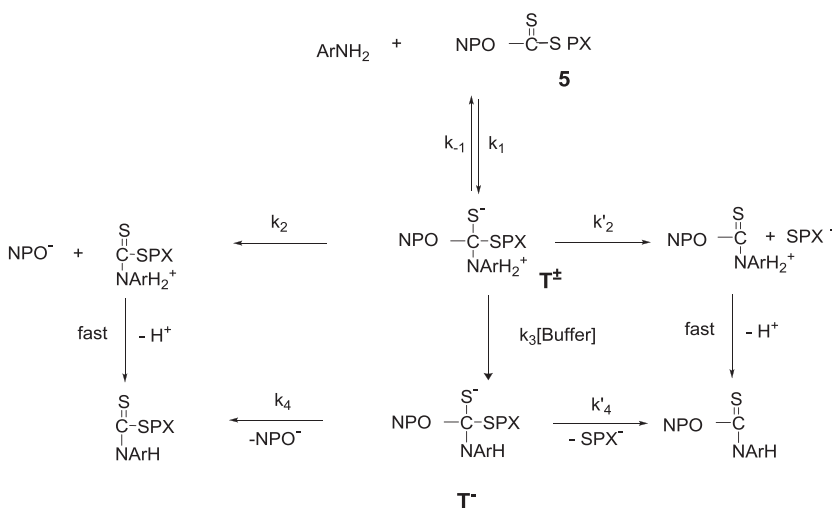
SCHEME 4 Zwitterionic tetrahedral intermediates in the reactions of 5 with anilines (I), SA amines (II), and pyridines (III)
