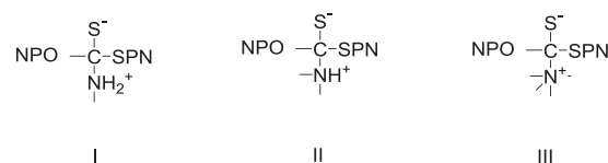
SCHEME 4 Zwitterionic tetrahedral intermediates in the reactions of 5 with anilines (I), SA amines (II), and pyridines (III)
