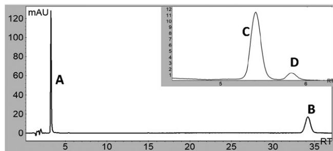
FIGURE 1 High-performance liquid chromatography analysis of the reaction of 5 with aniline (from 0 to 37 min, at \lambda = 316 nm). A, 4-nitrophenol. B, Dimer of 4-nitrobenzenethiol. The insert is a small part of the same chromatogram (4.5–6.5 min at \lambda = 270 nm). C, 4-Nitrobenzenethiol aniline dithiocarbamate. D, 4-Nitrophenyl aniline thiocarbamate
