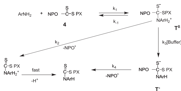
SCHEME 2 Proposed mechanism for the anilinolysis reactions of dithiocarbonate 4 , ( X=H )
