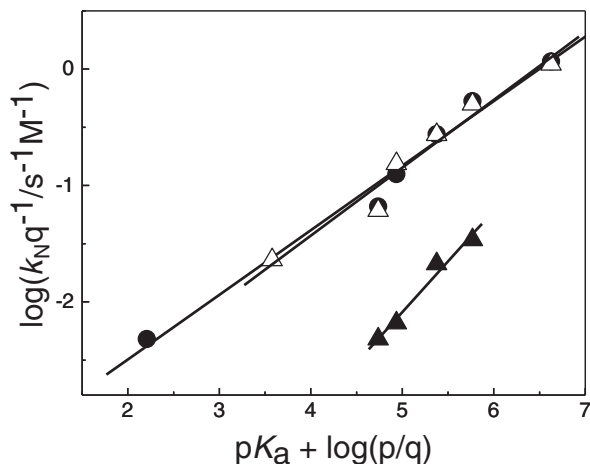
FIGURE 2 Corrected Brønsted-type plots for the anilinolysis of 4 (▲), 5 (●), and 6 (Δ)
