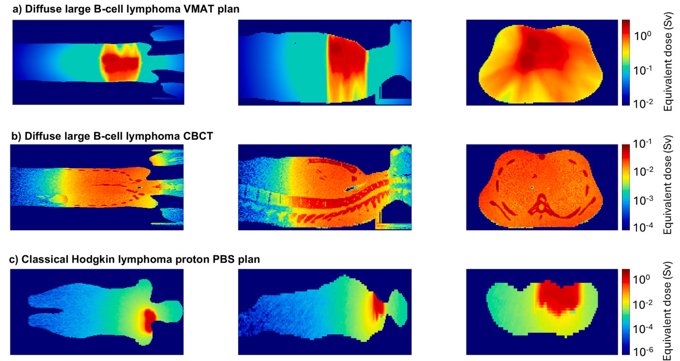
Fig. 4. Dose distribution in the diffuse large B-cell lymphoma (DLBCL) a) VMAT fraction, b) DLBCL CBCT fraction, and c) classical Hodgkin lymphoma proton PBS fraction (c). From left to right: coronal, sagittal and axial views at the isocenter plains.
