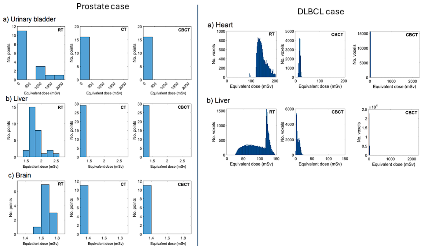
Fig. 5. Left panel: Pseudo-dose volume histograms (pDVHs) in the prostate case for the a) urinary bladder, b) liver and c) brain. pDVHs were built using the binning adjusted between the minimum and maximum dose received by each organ in the RT exposure. Right panel: DVHs in the diffuse large B-cell lymphoma VMAT case for the a) heart and b) liver. DVHs in first and second column were built using the binning adjusted between the minimum and maximum dose received by each organ in the RT exposure, while the representative binning from target was used in the third column.
