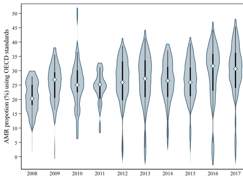
Fig. 1: Average proportion of resistance across antibiotic-bacterium pairs, based on annual reports from 39 participating hospitals in Chile (2008–2017). Notes: Antibiotic-bacterium pairs as defined by the OECD. 2 Violin plots present the probability density (distribution) of AMR rates at their different values. Density is smoothed by a kernel density estimator. The diamond marker represents the AMR rates' median, while the thick black box shows the interquartile range (the difference between 75th and 25th percentiles). The thin grey line indicates 95% CI.
