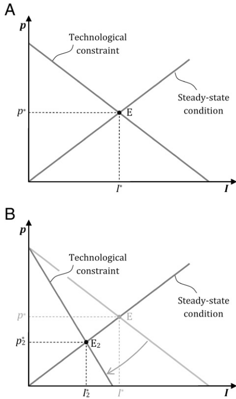
Fig. 3. Determination of the steady-state equilibrium values of I_t and p_t (panel A). When the child labor productivity rises, the technology constraint rotates inwards, and both I^* and p^* fall (panel B).
