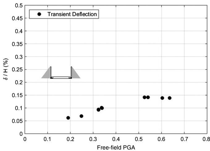
Fig. 7. Transient deflection of the nondisplacing retaining wall
