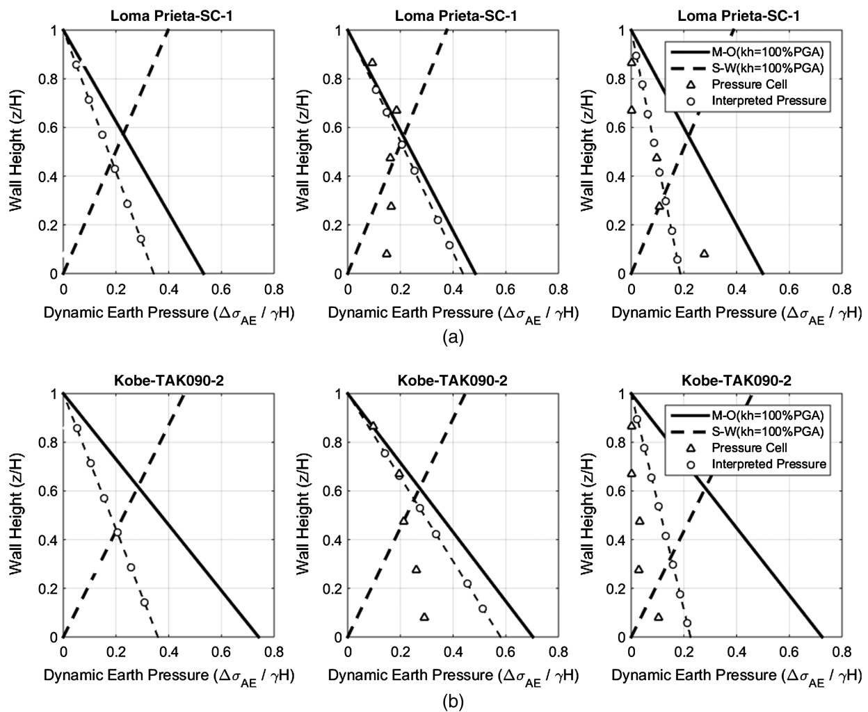
Fig. 4. Dynamic earth pressure distributions measured directly from the pressure sensors and strain gage, load cell data, and estimated M-O and S-W on walls for (a) Loma Prieta-SC-1 ( PGA_{ff} = 0.51g ); (b) Kobe-TAK090-2 ( PGA_{ff} = 0.61g )
