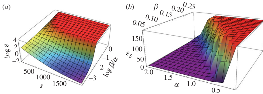
Figure 2. Efficient language evolves if the individual's cost of producing it is under a threshold level. (a) The evolution of noise level (communication efficiency) as a function of the ratio of the cost parameters. s denotes evolutionary time; \alpha and \beta denote the cost parameters (figure 1); and \varepsilon is the average noise level of the group. (b) Average noise level at the end of the evolutionary process as a function of the two cost parameters. The symbol \varepsilon_s denotes average noise level of the group at the end of the evolutionary process. (Average of 40 repeats, n = 10 , k = 4 , \tau = 40 , \varepsilon_0 = 10 , the variable \varepsilon ranges between 0 and 180.)
