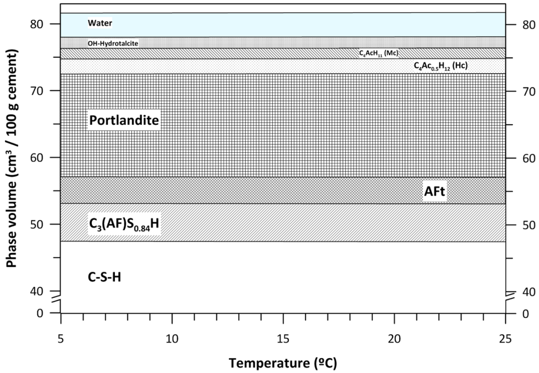
Figure 7. Predicted phase assemblage at thermodynamic equilibrium as a function of curing temperature determined for Chilean OPC cement at a w/c of 0.4.
