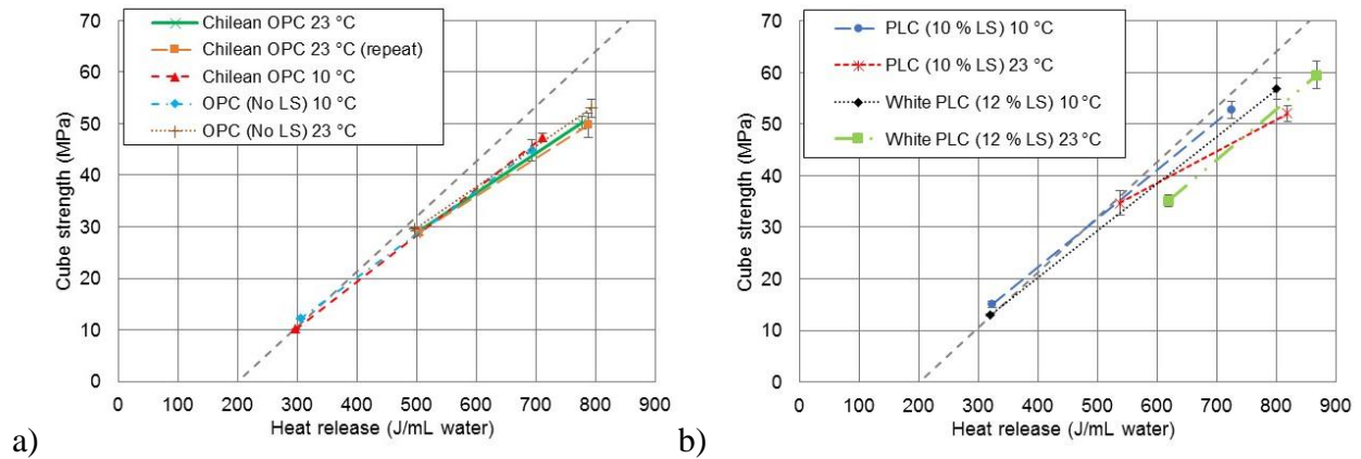
Figure 2. Cube compressive strength vs. heat release per unit volume of water for specimens cured at two temperatures and tested after 1 d and 7 d for: a) Chilean OPC with no LS and (US) OPC with no LS and b) PLC (10 % LS) and white PLC (12 % LS). For each plot, dashed grey line indicates strength-heat release relationship found for mortars in a previous study [11].
