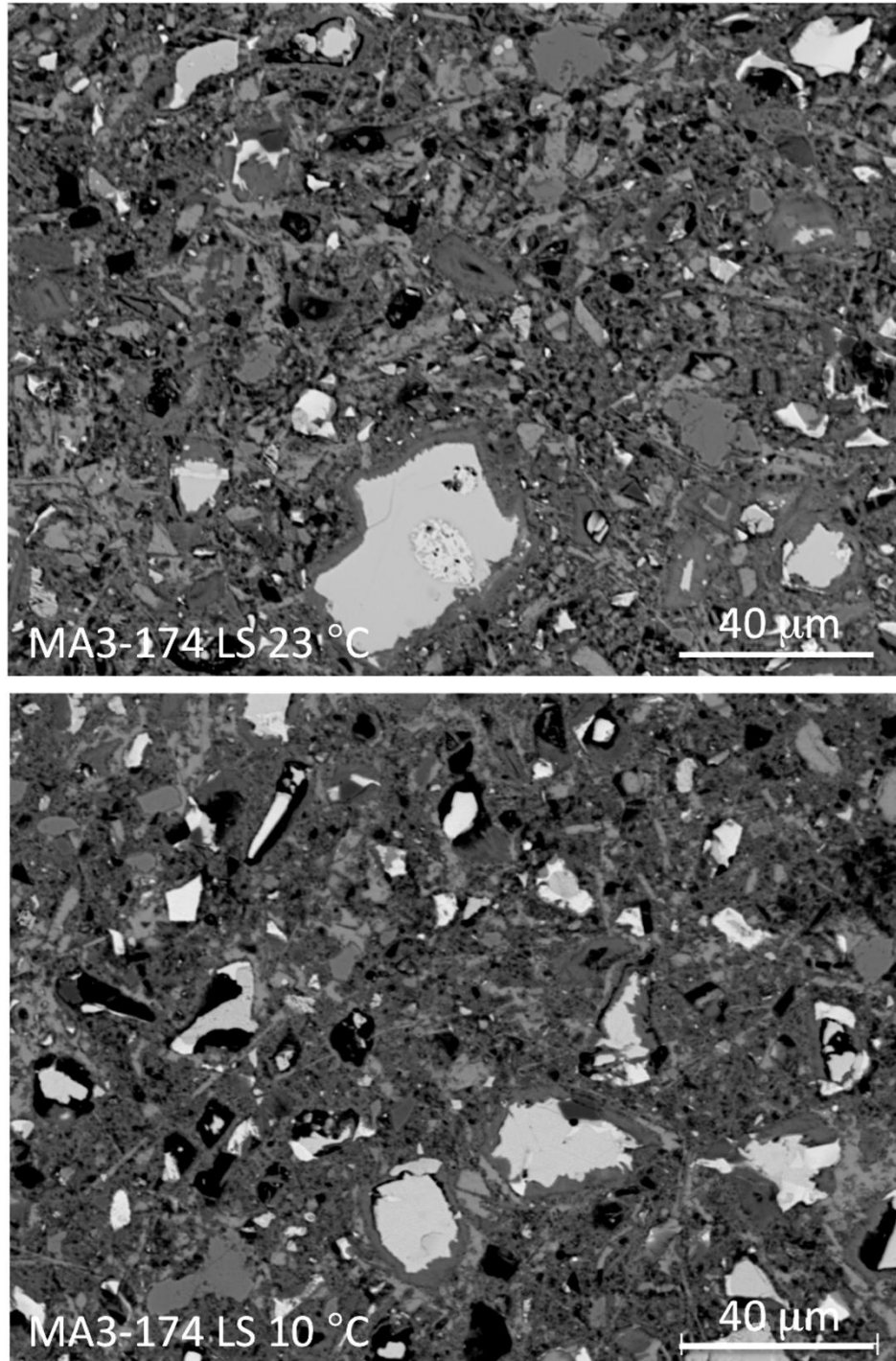
Figure 6. PLC (10 % LS) paste microstructure after 7 d curing at 23 °C (upper) and 10 °C (lower) appears to have a more finely-sized and uniformly distributed portlandite and for the 10 °C paste, a more dense-appearing C-S-H texture.
