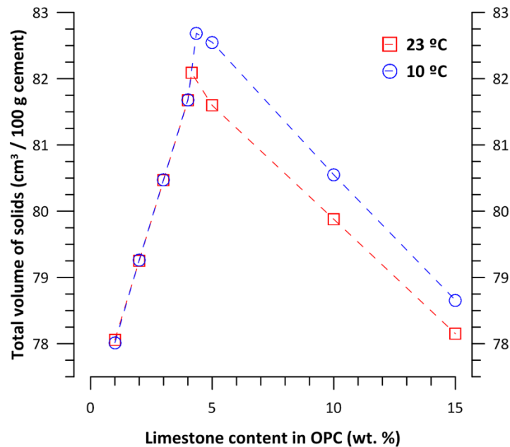
Figure 10. Effect of limestone replacement level on the total volume of solids of Chilean OPC at 10 °C and 23 °C. The optimum is shown as the maximum for each temperature.
