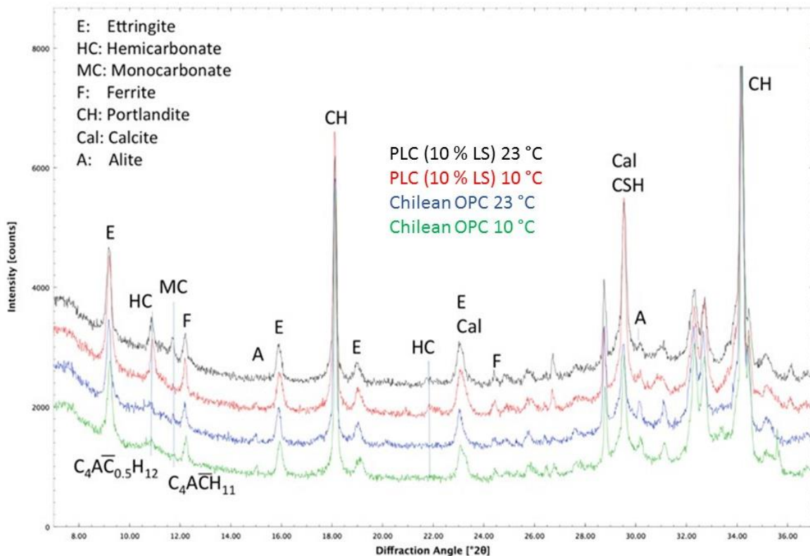
Figure 4. Low angle region of the 7-d X-ray powder diffraction patterns illustrates differences in HC and MC phases with sharper, better-ordered HC and MC in pastes from limestone-containing cement at both 10 °C and 23 °C. Patterns from bottom to top are Chilean OPC at 10 °C, Chilean OPC at 23 °C, PLC (10 % LS) at 10 °C, and PLC (10 % LS) at 23 °C.
