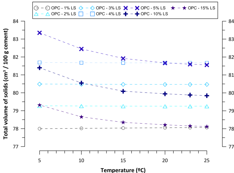
Figure 9. Effect of temperature on the total volume of solids at thermodynamic equilibrium of Chilean OPC with different amounts of limestone replacements.
