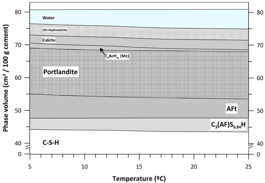
Figure 8. Predicted phase assemblage at thermodynamic equilibrium as a function of curing temperature determined for PLC (10 % LS) cement at a w/c of 0.4.
