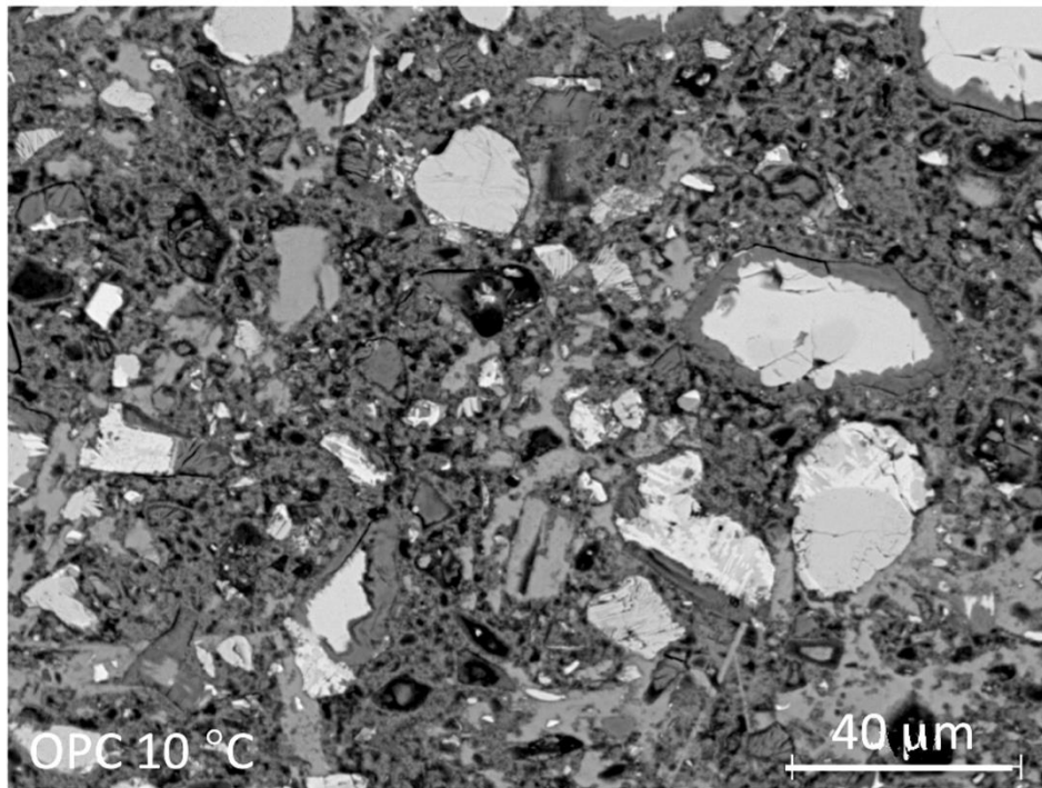
Figure 5. 7-d Chilean OPC cured at 23 °C (top) and 10 °C (bottom), showing (in order of brightness), residual cement grains (brightest), portlandite (CH), C-S-H and AFm, and voids (darkest).
