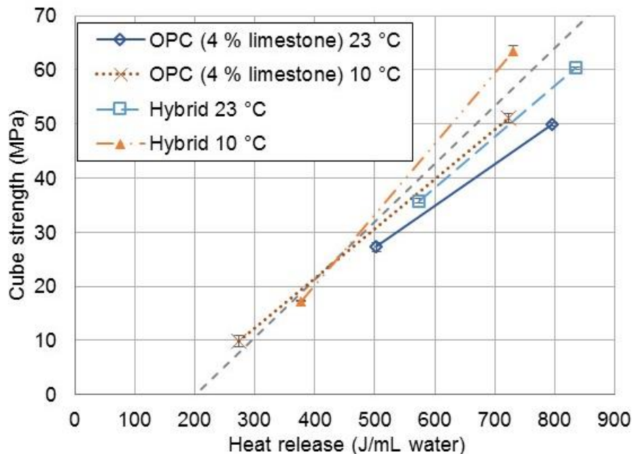
Figure 1. Mortar cube compressive strength vs. heat release per unit volume of water for an ASTM C150 Type I/II ordinary portland cement with a 4 % limestone addition and for a hybrid mortar containing 20 % limestone and 1 % \text{CaCl}_2 (both replacing sand) by mass of cement, cured at 10 °C or 23 °C (data from reference [8]). Error bars indicate \pm one standard deviation in measured compressive strength for 3 cube specimens. Dashed grey line extending from (200, 0) to (850, 70) indicates strength-heat release relationship found for mortars in a previous study [11]. At 7 d, absolute strength value is slightly higher for both mortars cured at 10 °C than for the corresponding ones cured at 23 °C.
